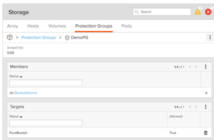
Figure 24. Targets displayed
