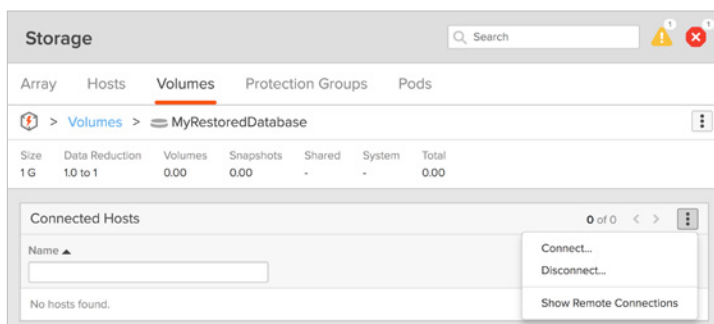
Figure 34. Connected hosts
