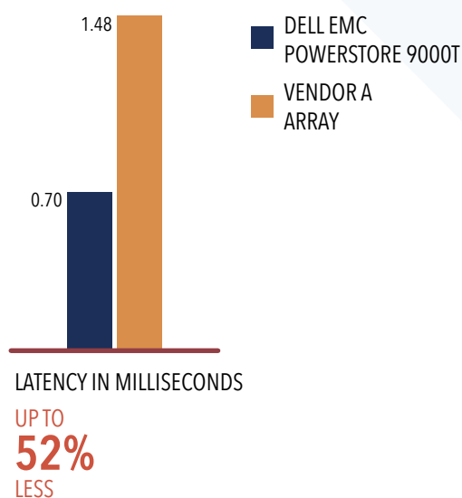
Figure 4: Response time (milliseconds) delivered while producing 360,000 IOPS. Lower is better. Source: Principled Technologies.
